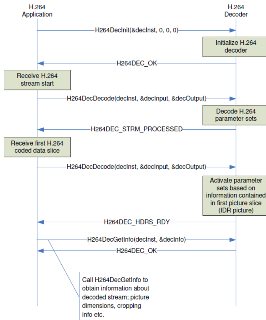
Figure 26. Simple Workflow Shown in the H.264 Example
