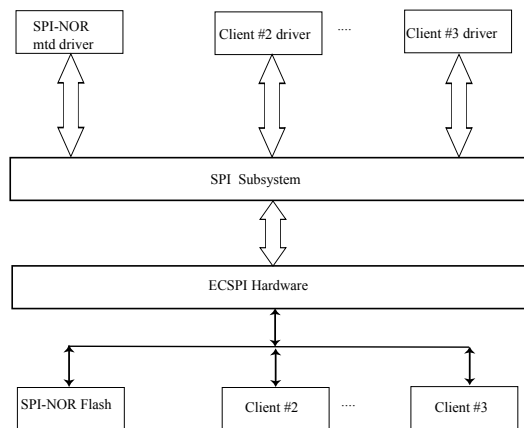
Figure 8. SPI Subsystem
