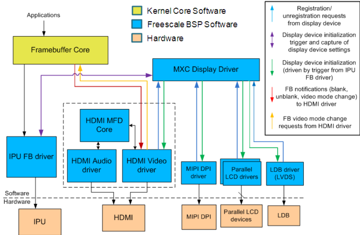
Figure 23. HDMI Video Software Architecture
